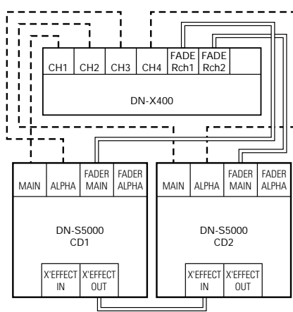
Fader start connections example 2
