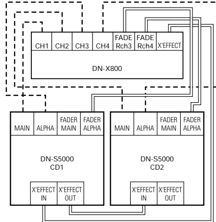
X-Effect connections example 2
